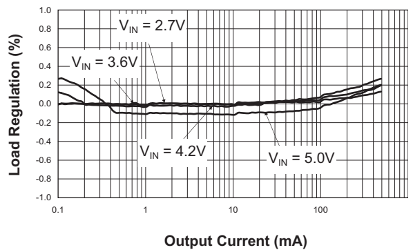
Load Regulation ( V_{OUT} = 1.2V ; L = 1.5\mu H )
